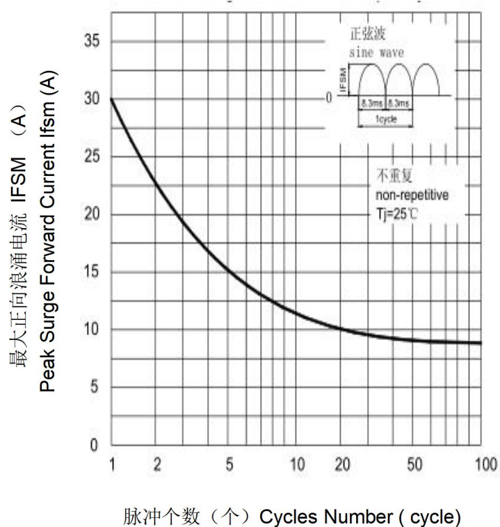
Fig.3: Forward Surge Current
